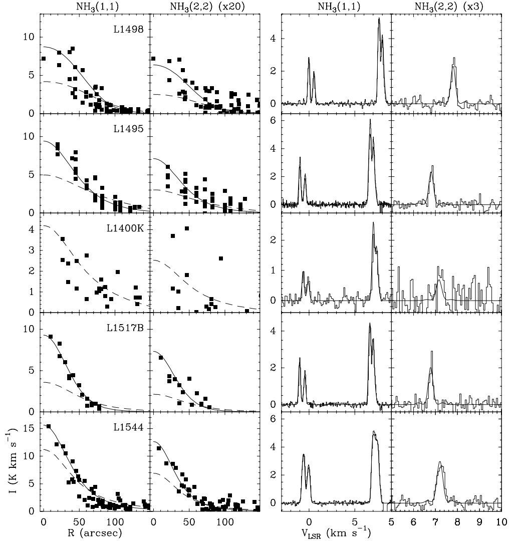
FIG. 6.— Radial profiles of \text{NH}_3(1,1) and (2,2) integrated emission (left) and central emerging \text{NH}_3(1,1) and (2,2) spectra (right). Observations are indicated by solid squares in the radial profiles (sum of all hyperfine components) and by histograms in the spectra (all temperature units are in the main beam scale). Dashed lines represent constant abundance models and solid lines represent models with a central abundance enhancement (see Table 5 for values). Note how in all cores but L1400K the models with constant \text{NH}_3 abundance fail to fit the central intensity (models have been set to fit outer core emission), while the models with a central abundance enhancement fit the data at all radii for both the (1,1) and (2,2) transitions. For the emerging spectra, only part of the hyperfine group is presented in order to show in detail the matching of the linewidth and the hyperfine contrast. To use the same velocity scale in all spectra, both data and model for L1400K have been shifted by 4 \text{ km s}^{-1} , and by 1 \text{ km s}^{-1} for L1517B.
